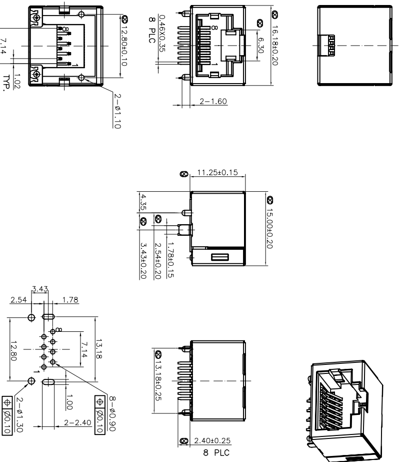
PC BOARD LAYOUT COMPONENT (THICKNESS:1.6mm) SIDE SHOWN
