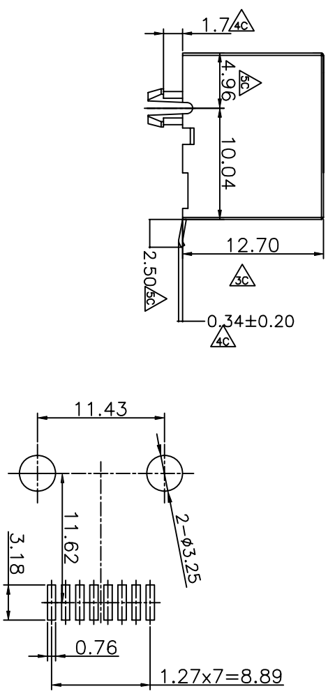
PCB LAYOUT/TOP VIEW
